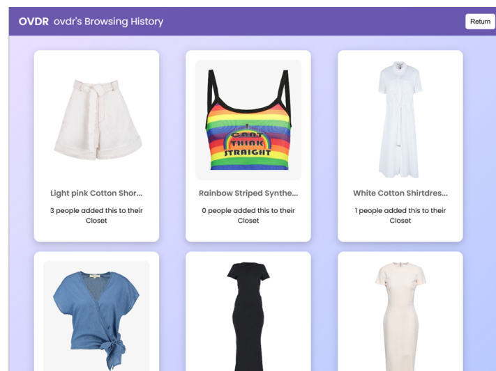
Figure 26: History Page
