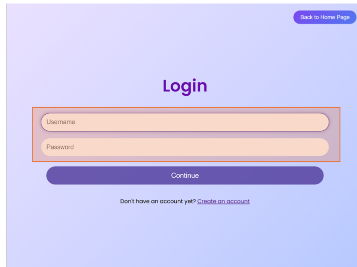
Figure 3: Login Page
