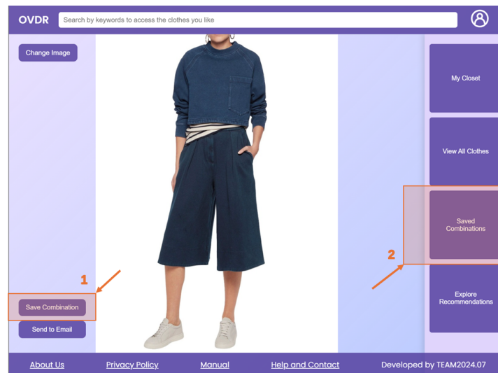
Figure 18: Save Combinations
