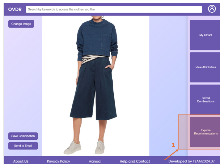
Figure 20: Get Recommendations
