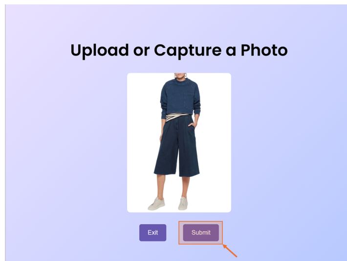
Figure 6: Submit Page
